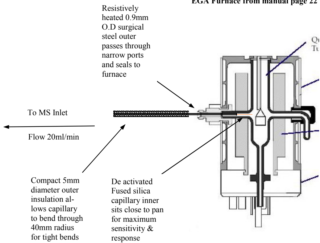
EGA Furnace from manual page 22
